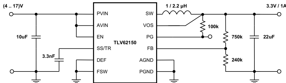
Figure 5. 3.3-V/1-A Step-Down Converter
