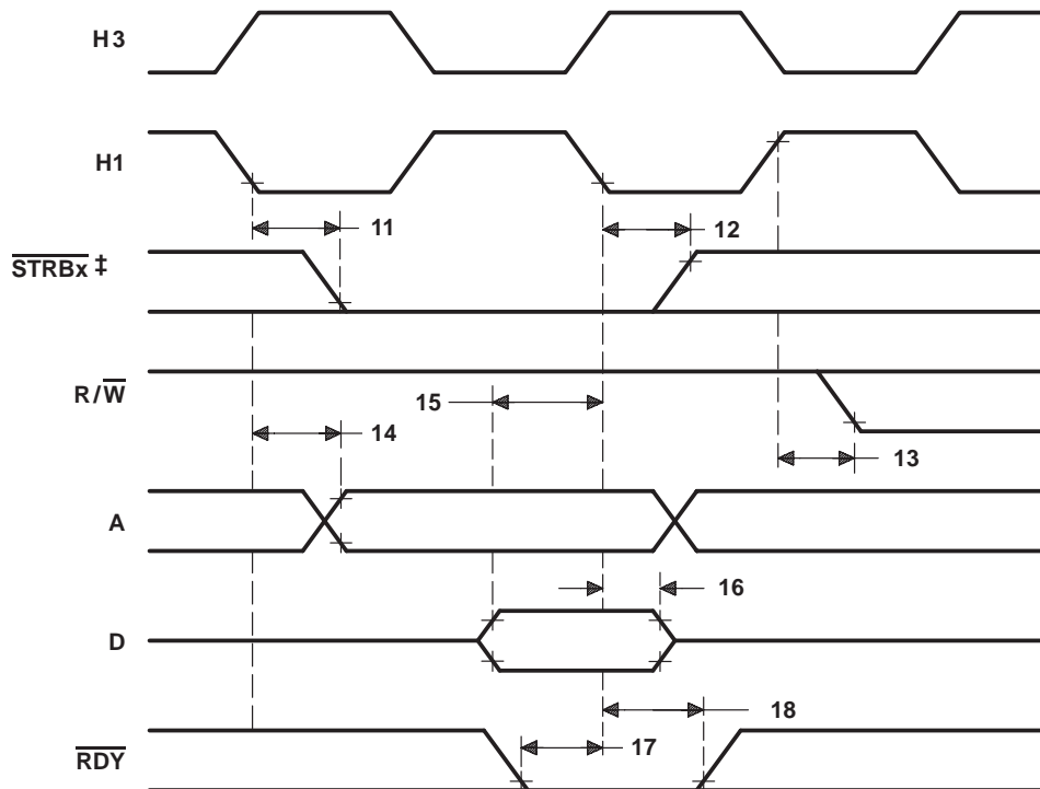
Figure 16. Memory-Read-Cycle Timing
