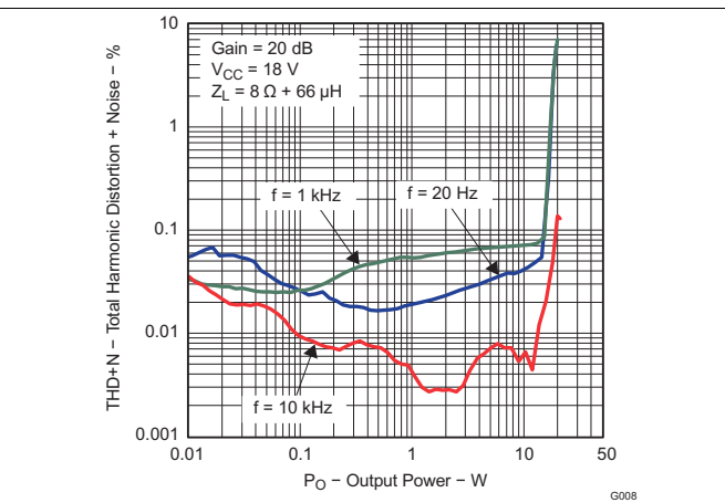
Figure 8. Total Harmonic Distortion + Noise vs Output Power (BTL)
