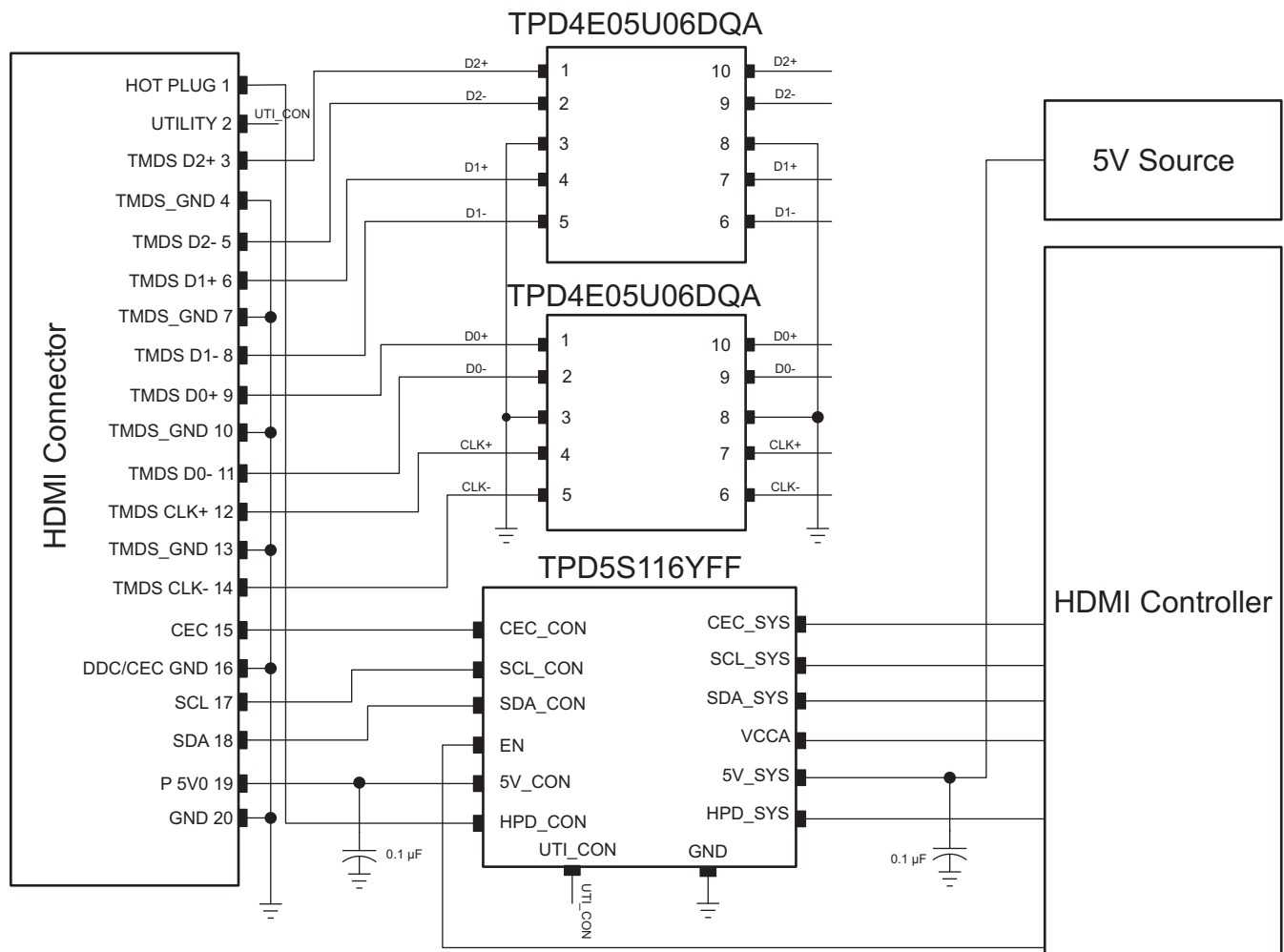
Figure 14. HDMI 2.0 Schematic
