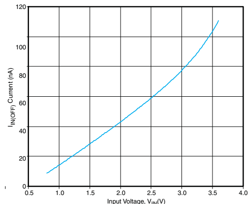
Figure 6. I IN(OFF) vs V IN (V ON = 0 V)
