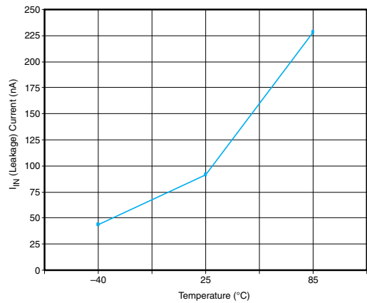
Figure 9. I_{IN} (Leakage) vs Temperature ( V_{IN} = 3.3\text{ V} )
