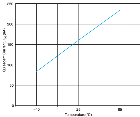
Figure 5. Quiescent Current vs Temperature (V IN = 3.3 V, I OUT = 0)
