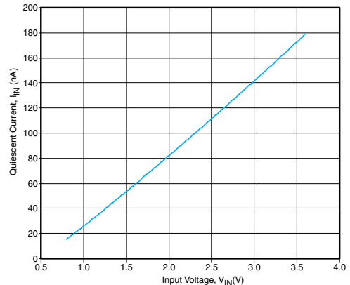
Figure 4. Quiescent Current vs V IN (V ON = V IN , I OUT = 0)
