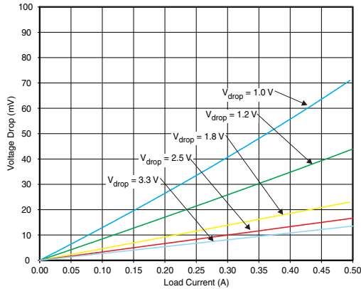
Figure 3. Voltage Drop vs. Load Current
