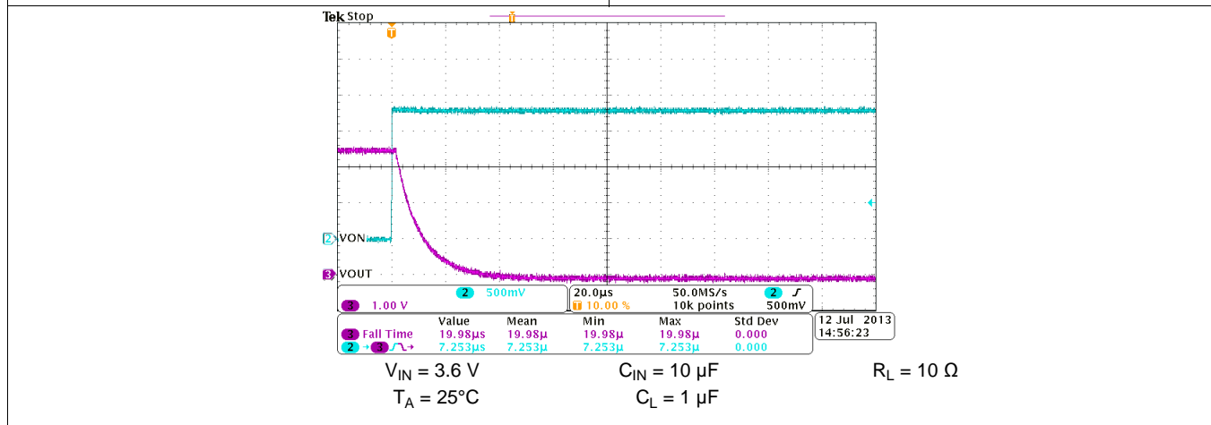
Figure 40. Turn-Off Response
