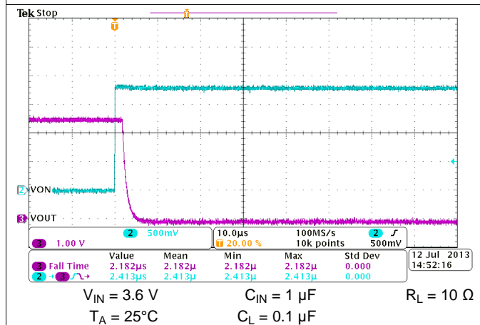
Figure 38. Turn-Off Response
