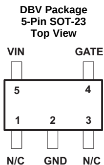
Pin Functions
