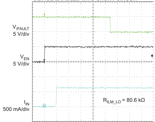
t - Time - 2 ms/div
