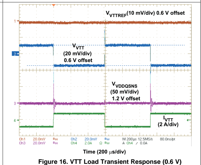
Figure 16. VTT Load Transient Response (0.6 V)
