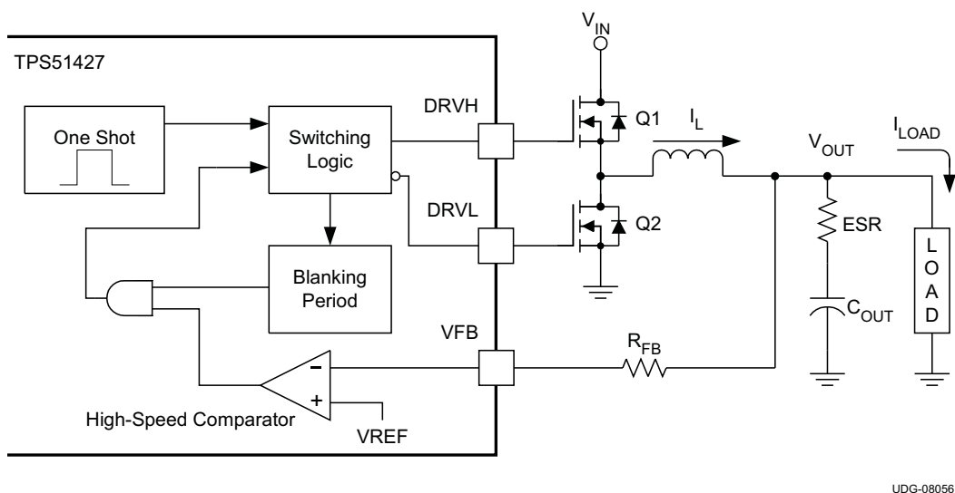
Figure 44. D-CAP Mode Operation Schematic
