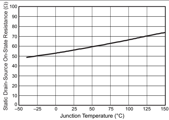
Figure 19. PWRGD On-Resistance vs Temperature
