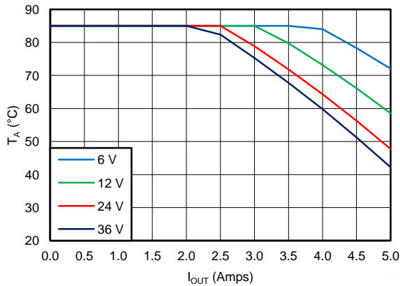
Figure 58. 3.3V Outputs
