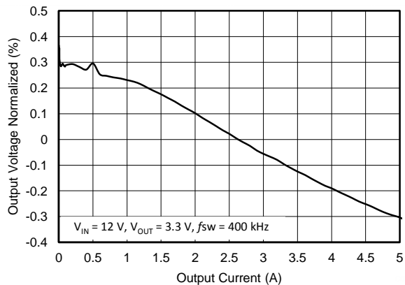
Figure 56. Regulation vs Load Current
