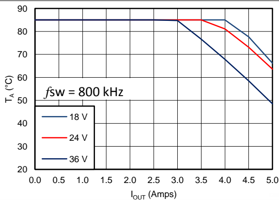
Figure 60. 12V Outputs
