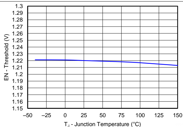
Figure 11. EN Terminal Voltage vs Junction Temperature
