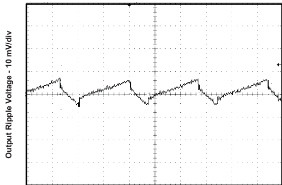
t - Time = 1 \mu s/div V_I = 5 V V_O = 3.3 V 6 A, 350 kHz
