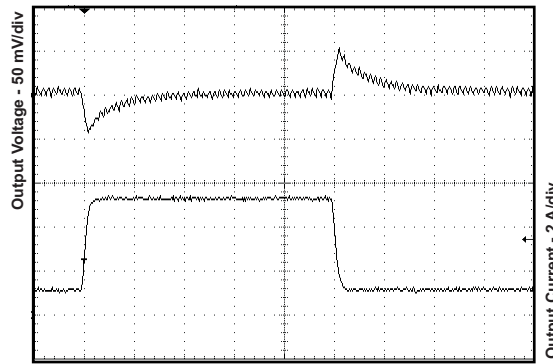
t - Time = 100 \mu s/div V_I = 5 V 1 A to 5 A
