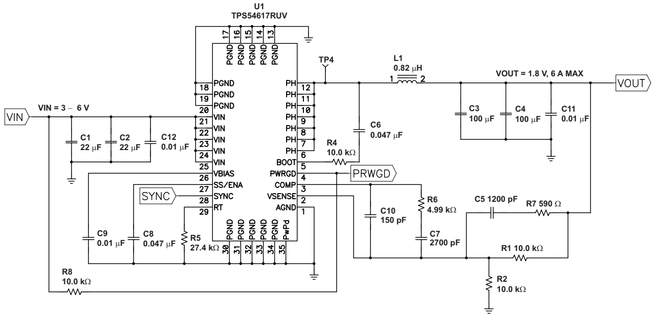
Figure 10. Application Circuit
