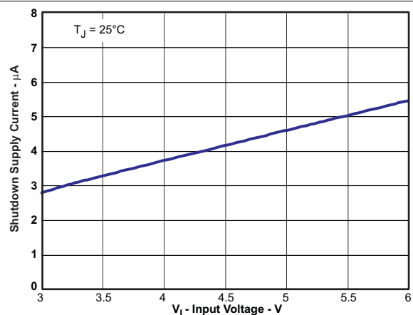
Figure 15. Shutdown Supply Current vs Input Voltage
