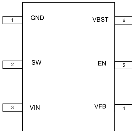
Pin Functions
