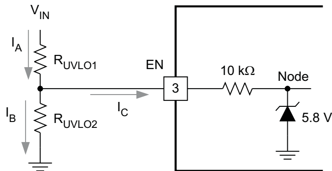
Figure 30. Node Voltage
