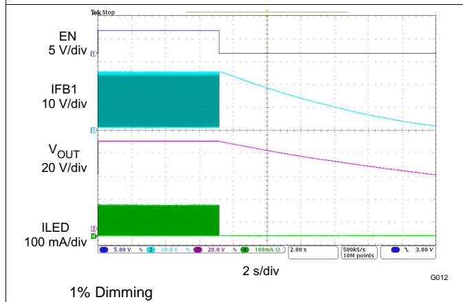
Figure 9. Dimming Waveform
