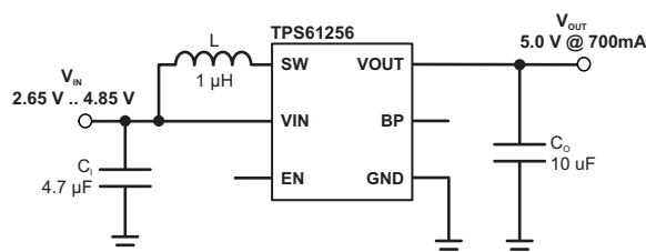
Figure 28. Smallest Solution Size Application
