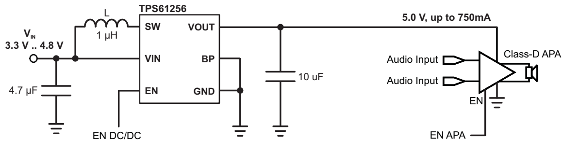
Figure 41. "Boosted" Audio Power Supply
