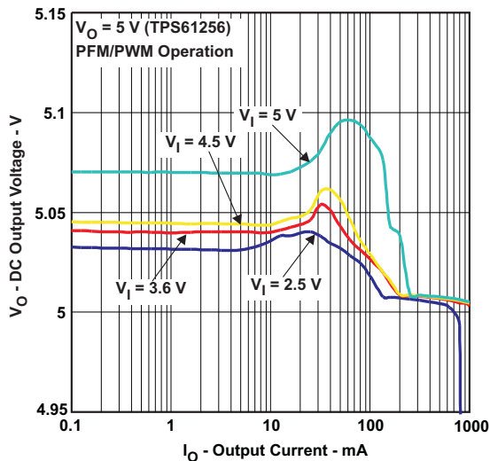
Figure 7. DC Output Voltage vs Output Current
