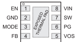
DSG Package 8-Pin WSON With Thermal Pad (Top View)
