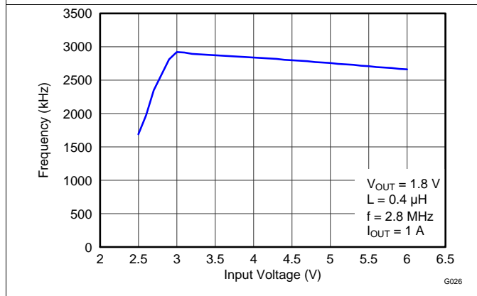
Figure 3. Switching Frequency vs Input Voltage
