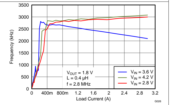
Figure 2. Switching Frequency vs Load Current
