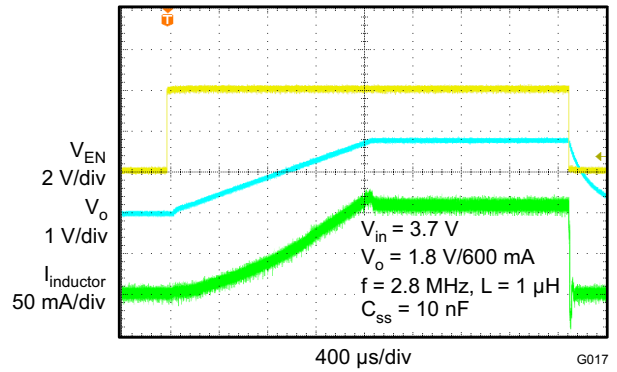
Figure 23. Start-Up
