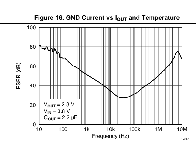
Figure 18. Power-Supply Rejection Ratio vs Frequency
