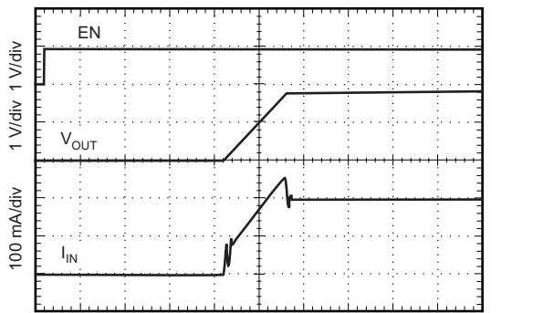
V_{IN} = 2.1 V V_{OUT} = 1.8 V I_{OUT} = 200 mA
