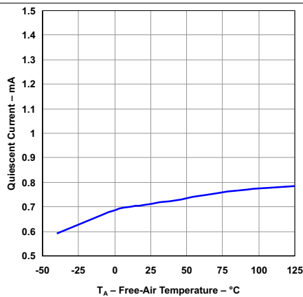
V_{IN} = 6\text{ V} V_{EN} = V_{IN} I_{OUT} = 0\text{ A} TPS73801
