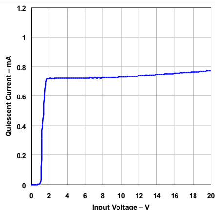
T_J = 25\text{ °C} V_{EN} = V_{IN} R_{OUT} = 4.3\text{ k}\Omega TPS73801
