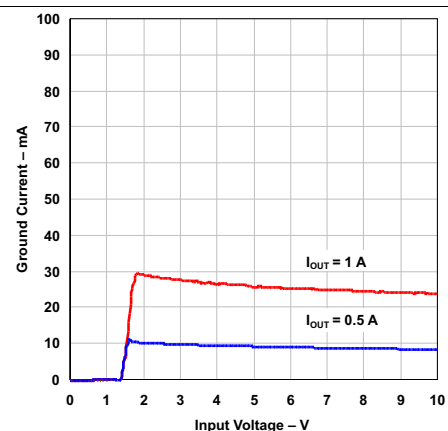
T_J = 25\text{ °C} V_{EN} = V_{IN} V_{OUT} = 1.21\text{ V} TPS73801
