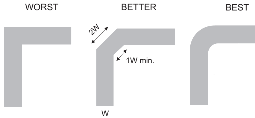
Figure 28. Trace Example
