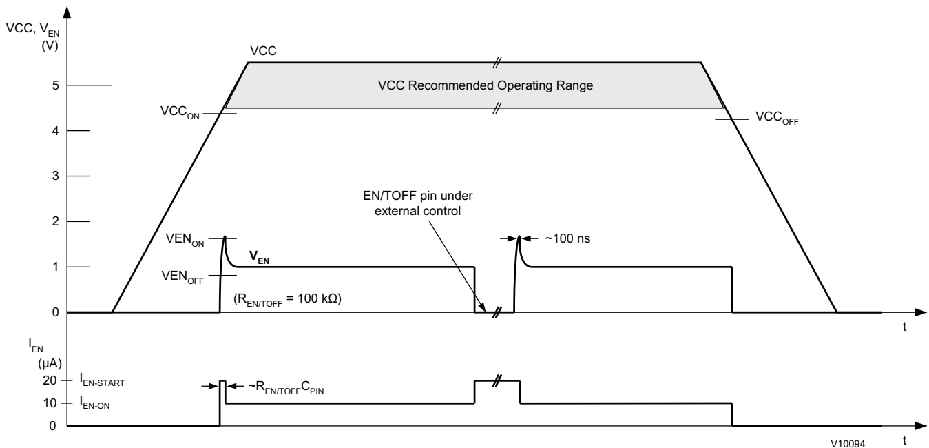
Figure 17. Behavior of I_{EN} and V_{EN} as V_{CC} Varies ( R_{EN/TOFF} = 100 k \Omega )
