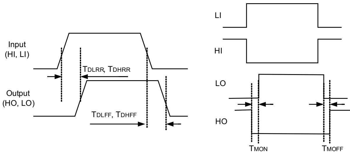
Figure 22. Timing Diagrams
