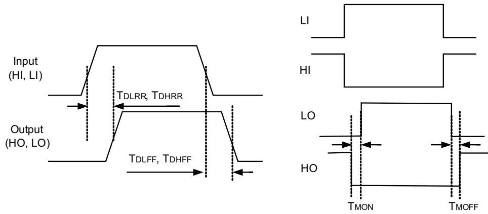
Figure 1. Timing Diagrams
