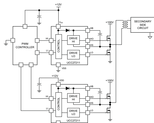
Typical Application: UCC27211
