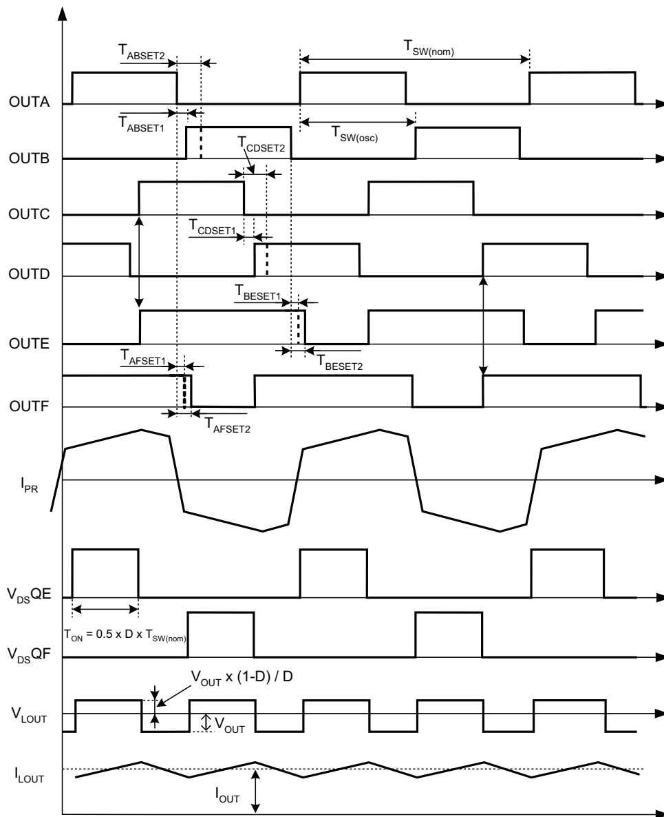
Figure 46. Major Waveforms of Phase-Shifted Converter
