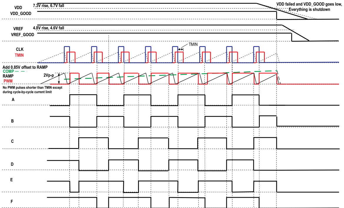
Figure 2. UCC28950 Steady State/Shutdown Timing Diagram
