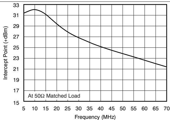
Figure 62. 2-Tone, 3rd-Order Intermodulation Intercept
