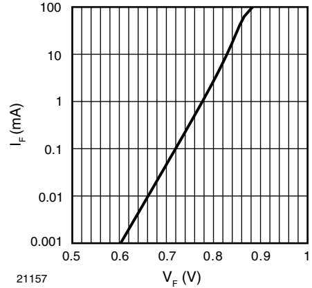
21157 Fig. 4 - Typical Forward Current I_F vs. Forward Voltage V_F
