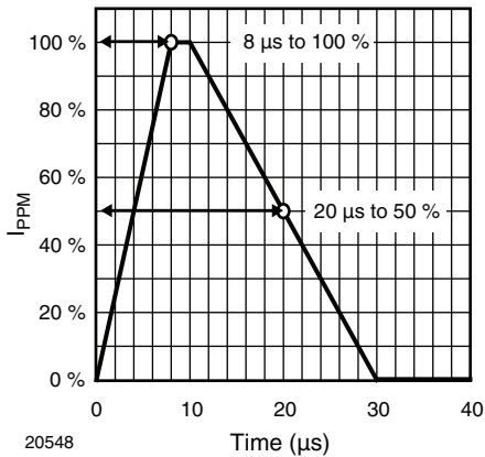
20548 Fig. 2 - 8/20 \mu\text{s} Peak Pulse Current Wave Form acc. IEC 61000-4-5
