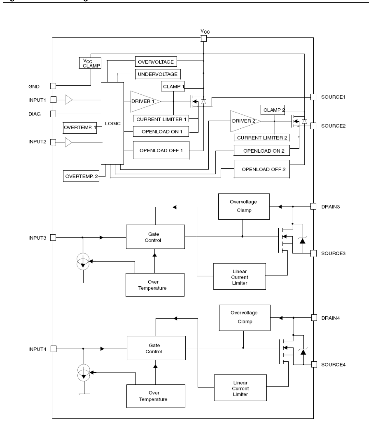
Figure 1. Block diagram
