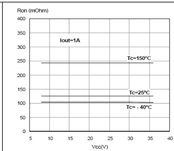
Figure 17. On-state resistance vs V_{CC}
