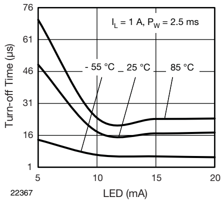
Fig. 10 - Turn-off Time vs. LED
