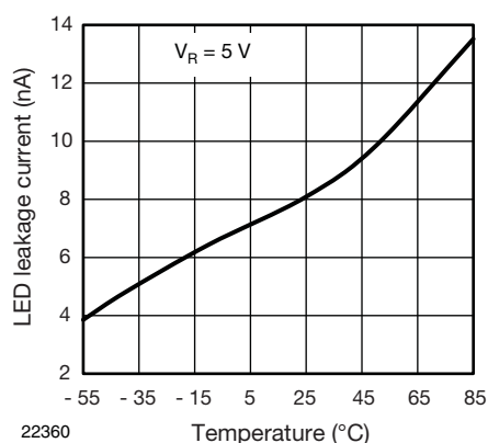
Fig. 3 - LED Leakage Current vs. Temperature
