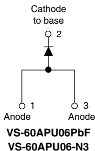
TO-247AC
