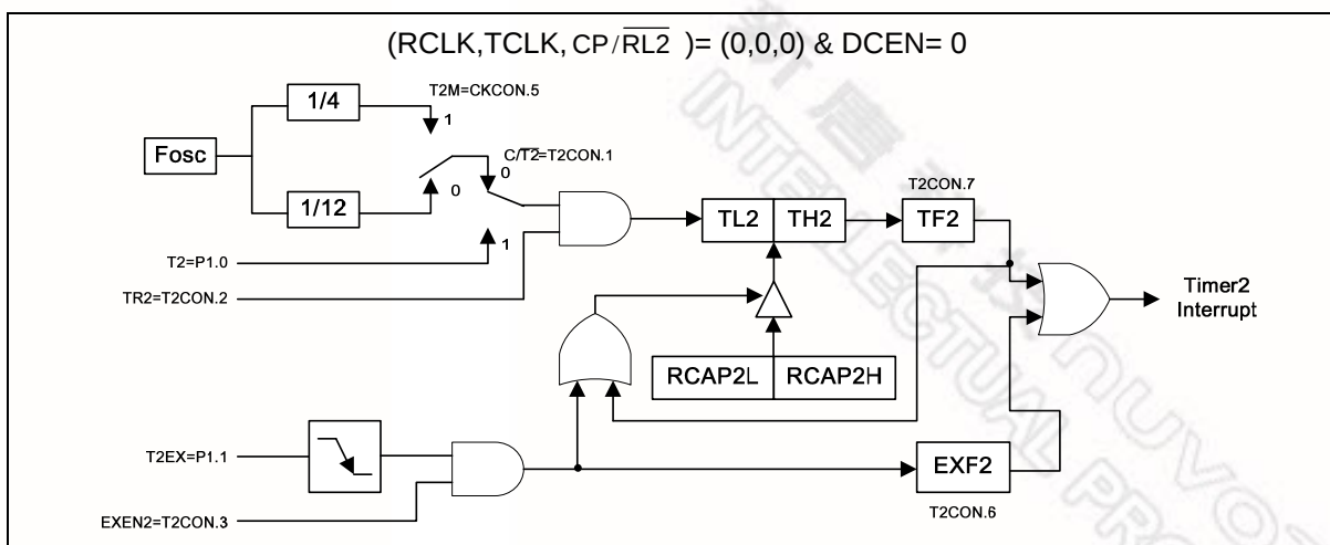
Figure 11-5 16-Bit Auto-reload Mode, Counting Up
