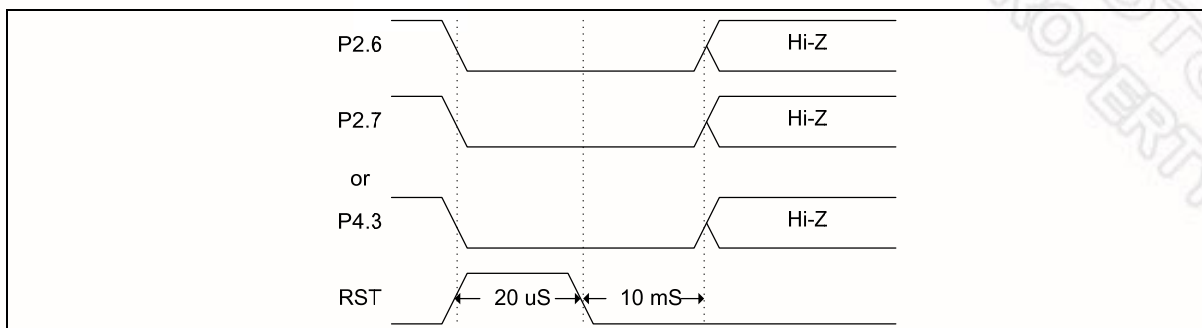
Figure 19-1 Timing of Entering Re-Boot Mode
