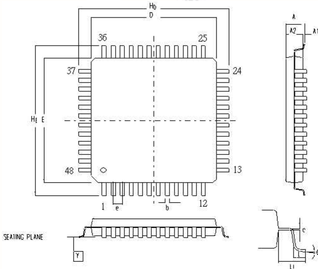
Controlling dimension : Millimeters
