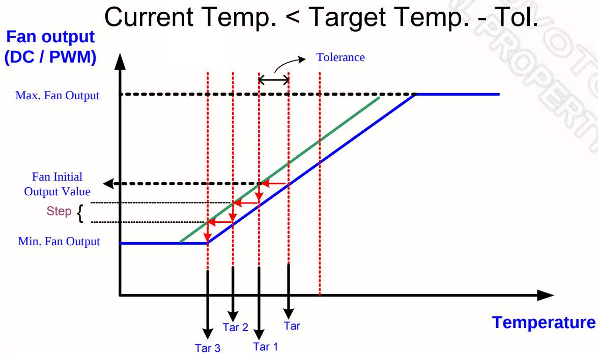
Figure 8-12 SMART FAN™ III Mechanism (Current Temp. &lt; Target Temp. - Tol.)
