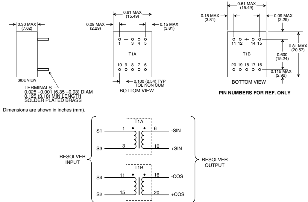
FIGURE 7. TRANSFORMER LAYOUT AND SCHEMATIC (RESOLVER INPUT - 52036/52037/52038)
