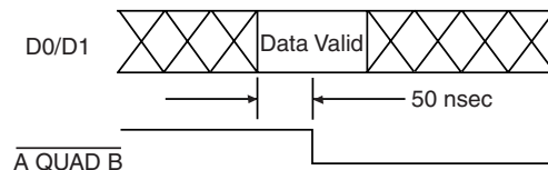
FIGURE 23. TIMING FOR INCREMENTAL ENCODER EMULATION RESOLUTION CONTROL
