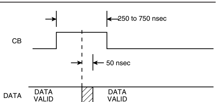
FIGURE 20. CONVERTER BUSY TIMING
