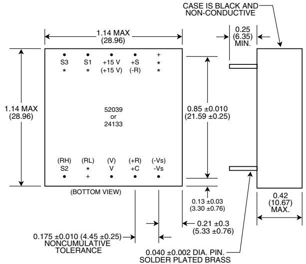
FIGURE 9. 60 HZ SYNCHRO AND REFERENCE TRANSFORMER DIAGRAMS (SYNCHRO INPUT - 52039 / REFERENCE INPUT - 24133)
