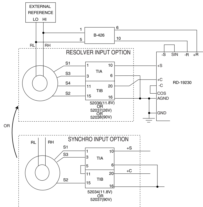
FIGURE 10. TYPICAL TRANSFORMER CONNECTIONS
