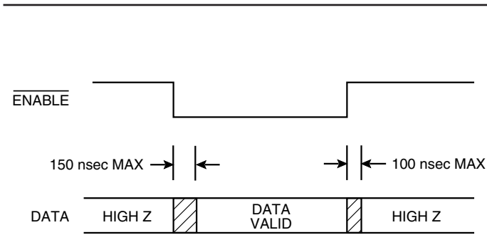
FIGURE 19. ENABLE TIMING
